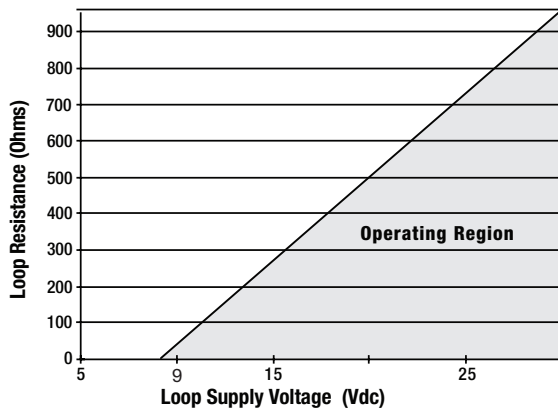
Loop Supply Voltage vs. Loop Resistance
